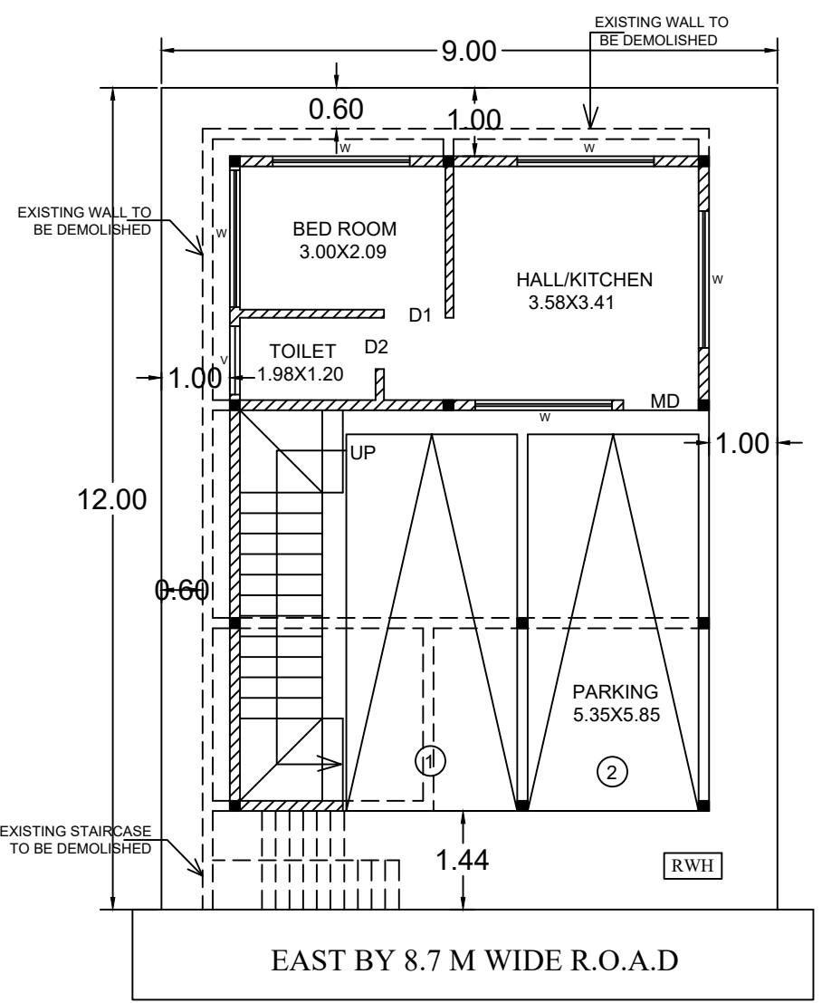
ALTERATION IN EXISTING GROUND FLOOR PLAN
